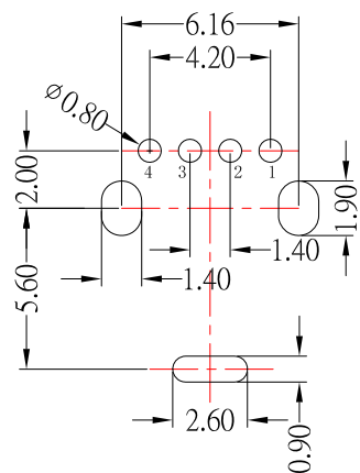
PCB LAYOUT MOUNTING PATTERN
